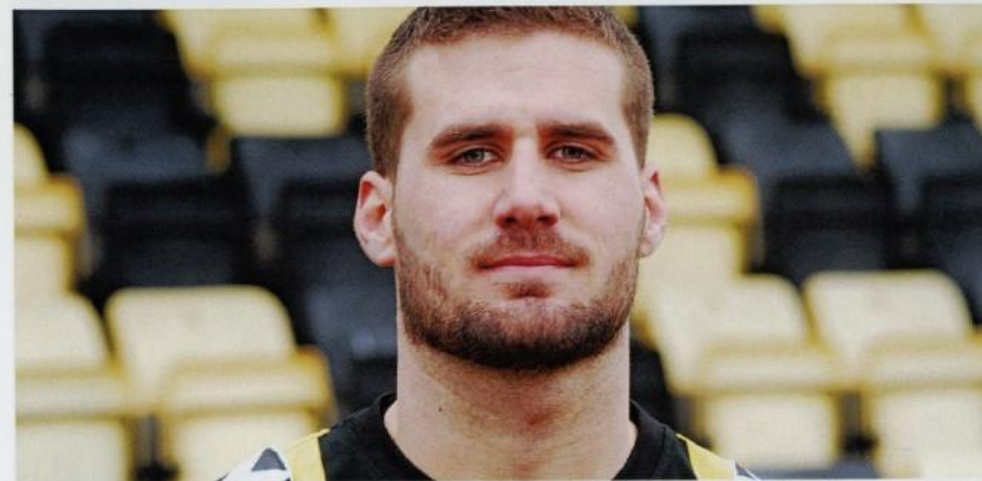
Sebastian scorede
